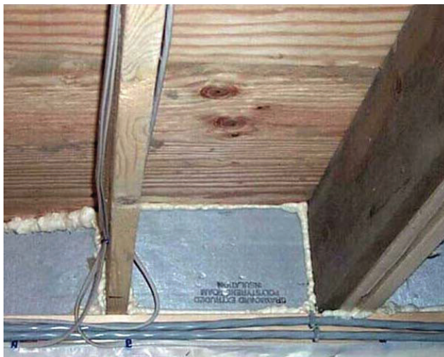
One-two part foam sill box.
