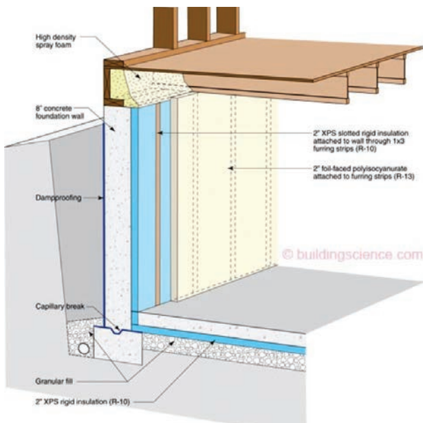
Basement and crawlspace insulation interior wall treatment.
