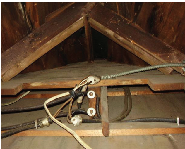
Knob and tube wiring.
