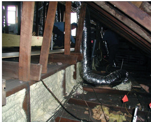
Ceiling height transition wall sealed with two-part foam.
