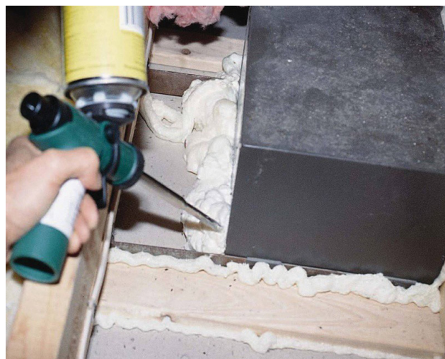
Bath fan sealed with one-part foam.
